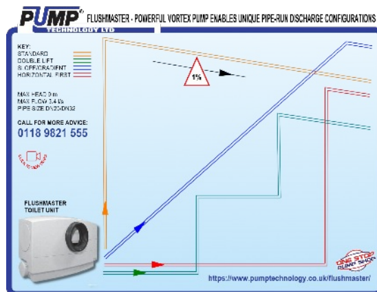
FlushMaster (Single toilet, shower and washbasin. Pumps convoluted discharge pipe runs)
